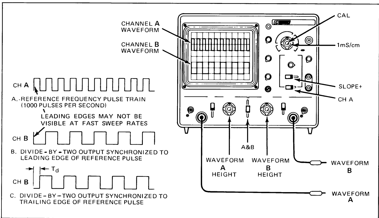
Fig. 8. Waveforms in divide-by-two circuit.
