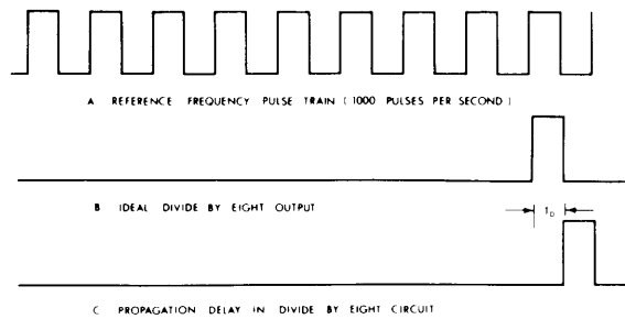
Fig. 9. Waveforms in divide-by-eight circuit.
