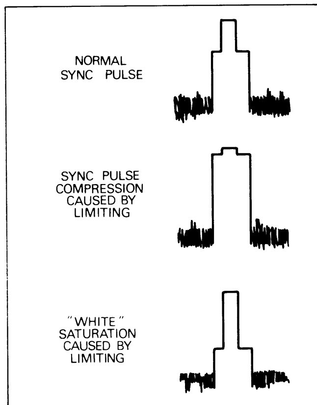
Fig. 24. Sync pulse waveforms.
