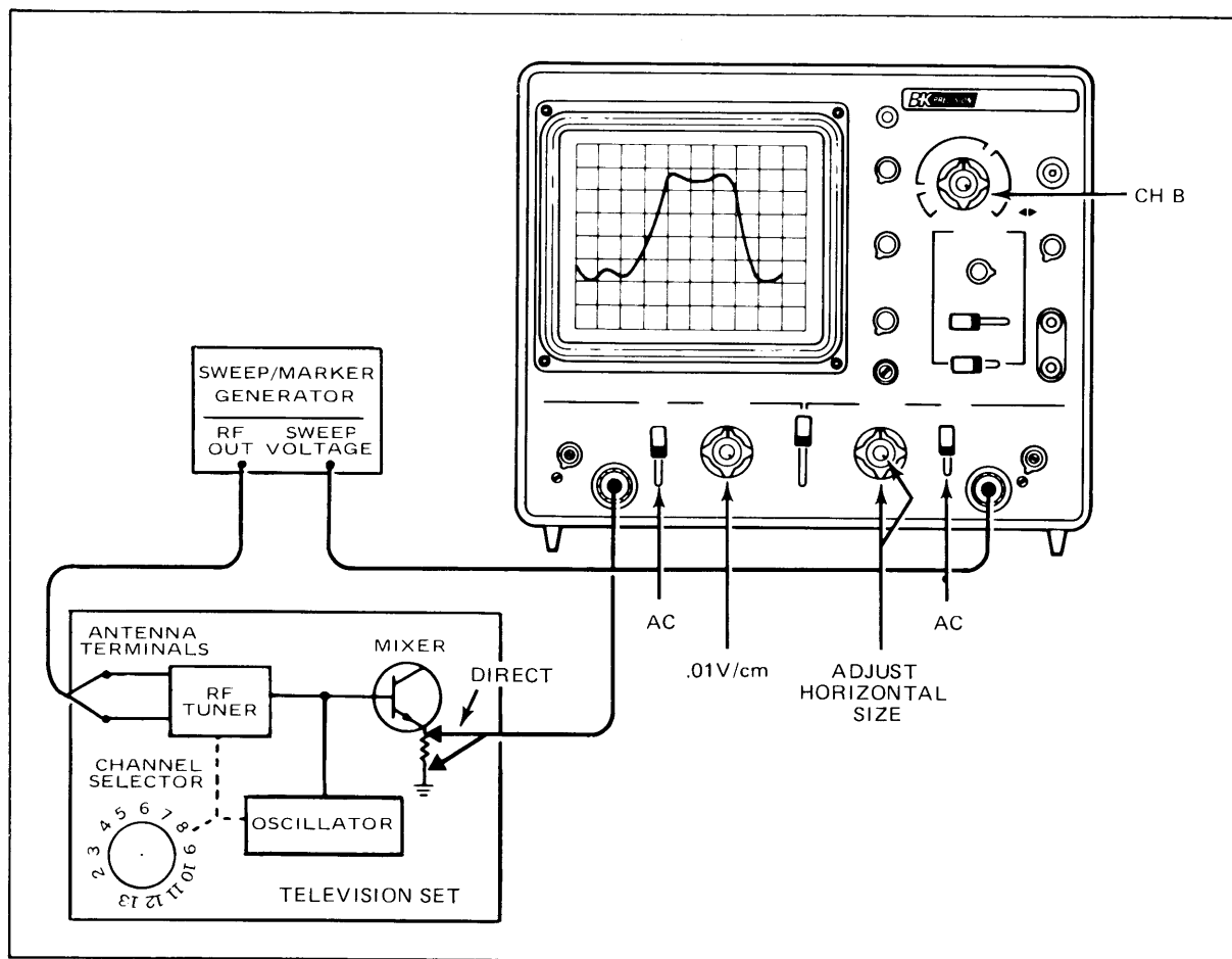
Fig. 33. Typical tuner alignment set-up.
