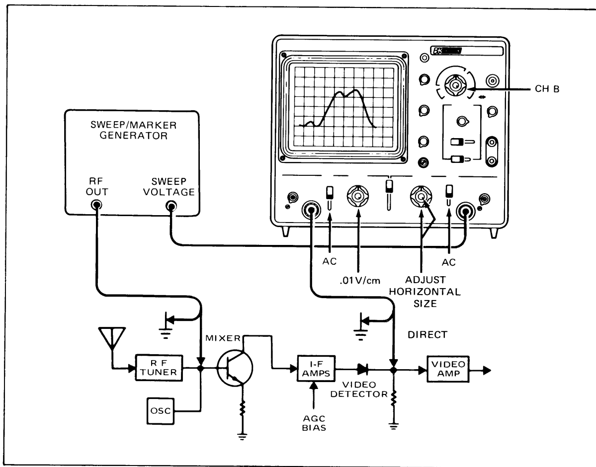
Fig. 34. Typical IF alignment set-up.
