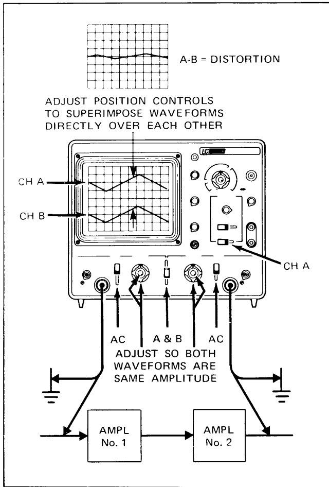
Fig. 13. Distortion measurement.
