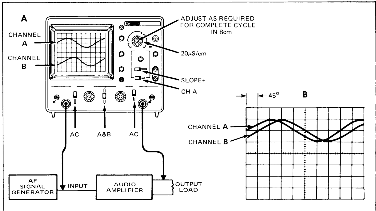
Fig. 18. Measuring amplifier phase shift.
