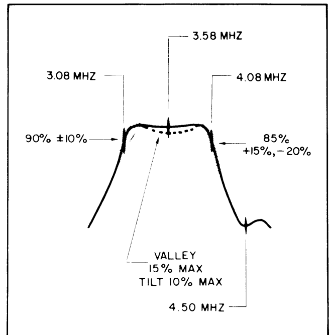
Fig. 37. Typical chroma response curve, showing tolerance ranges of response levels.
