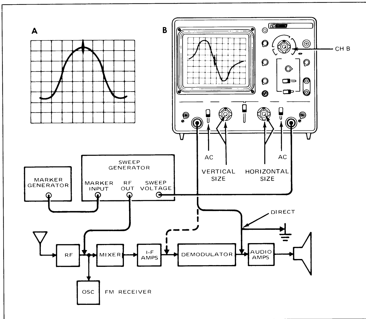
Fig. 38. Typical FM receiver alignment set-up.
