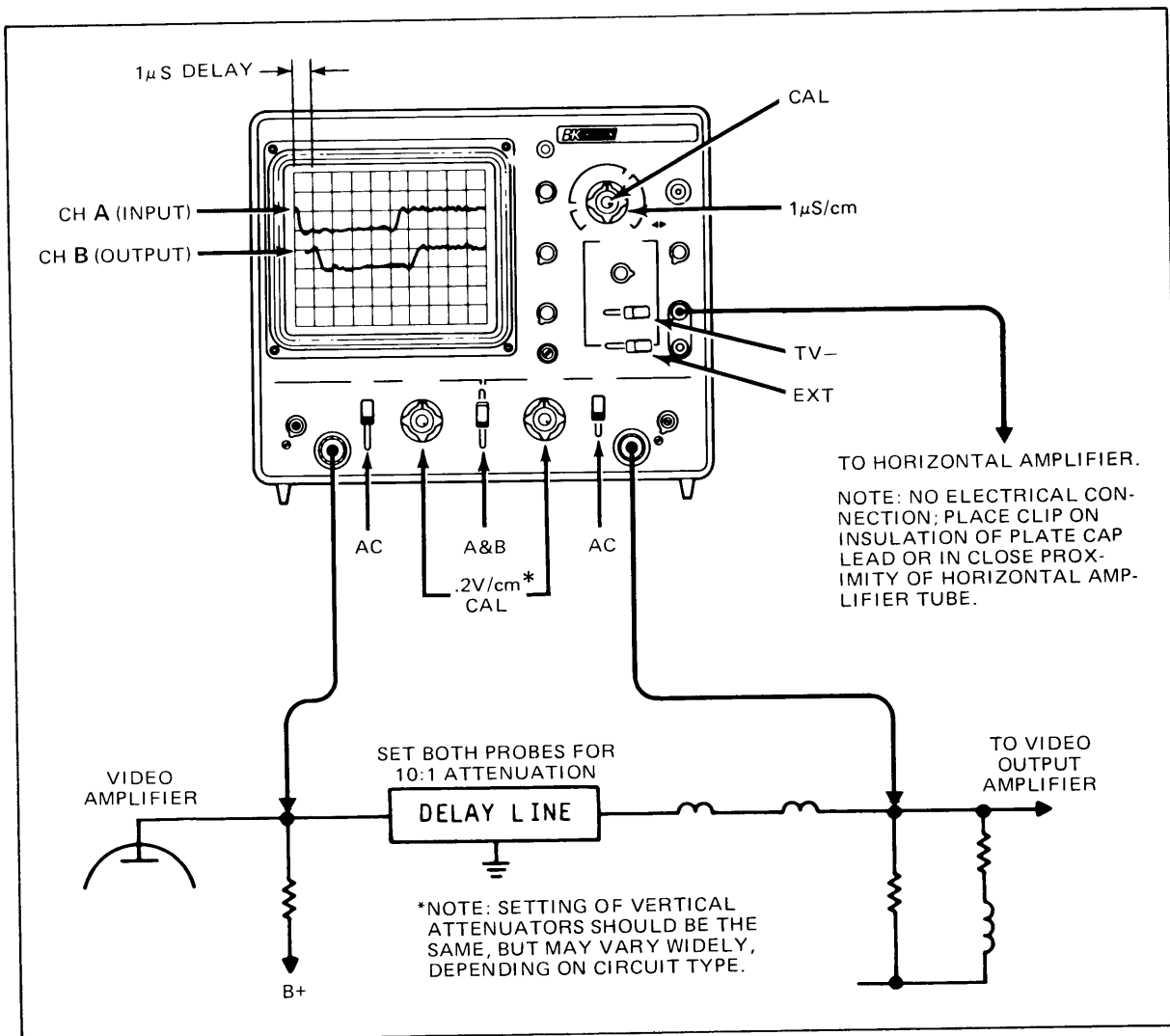
Fig. 16. Checking "Y" delay line in color television receivers.
