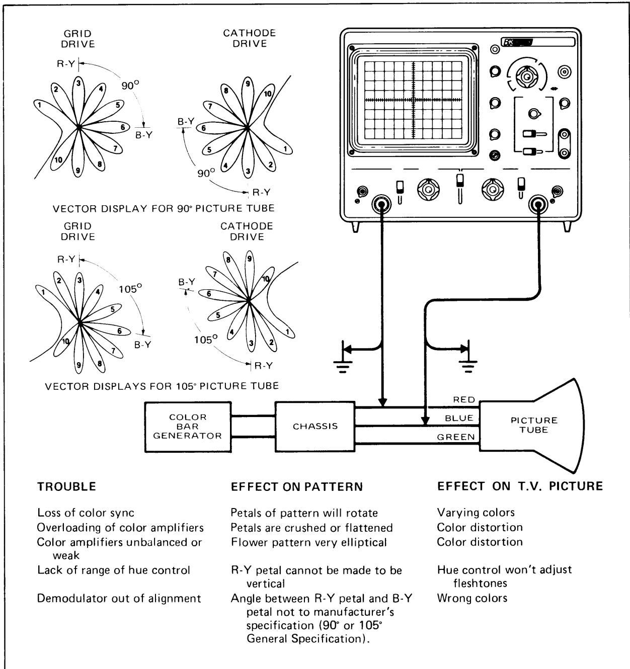
Fig. 31. Vectorscope operation and patterns.
